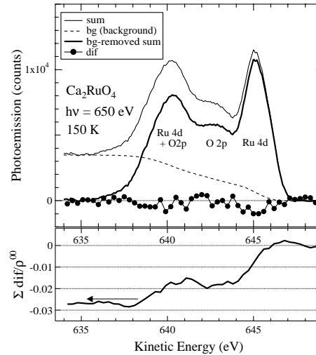
FIG. 4. Valence-band photoemission spectra of \text{Ca}_2\text{RuO}_4 . The thin solid curve and closed circles show the sum and difference of the spectra taken with parallel and antiparallel alignment. The dashed curve and thick solid curve indicate the background due to secondary electrons and the background-removed sum spectrum, respectively. In the lower panel, the difference spectrum normalized to \rho^{00} is integrated from the higher kinetic energy side.
