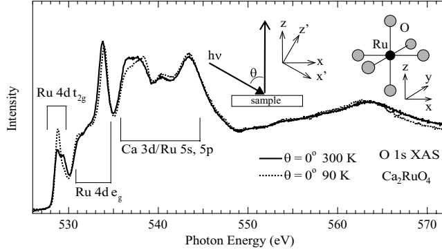
FIG. 1. O 1s x-ray absorption spectra of \text{Ca}_2\text{RuO}_4 taken at 90 K and 300 K at normal incidence. The spectra are normalized using the higher energy region above 550 eV. The insets show schematic pictures of the experimental arrangement and the \text{RuO}_6 octahedron.
