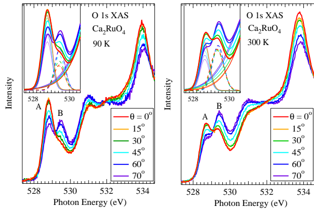
FIG. 2. O 1s x-ray absorption spectra of \text{Ca}_2\text{RuO}_4 taken at 90 K and at 300 K as a function of angle \theta , which is the angle between the surface normal and the Poynting vector of the circularly polarized light. The spectra are normalized using the higher energy region above 550 eV. In the insets, the fitted results are shown by the thick solid curves. The two Gaussians for structures A and B, and the tail of another Gaussian for the e_g band are shown by the dotted, dashed, and solid curves, respectively.
