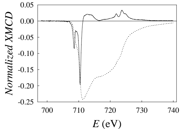
Fig. 4 – XMCD signal, normalized at unit white line intensity at the L-III edge for the Fe8 compound (full line). The field is 7 T and temperature is 4 K. The dotted line is the integrated XMCD.
