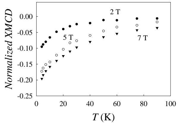
Fig. 2 – Normalized XMCD intensity for the peak at c.a. 710 eV in Fe8 as a function of T and at different fields.
