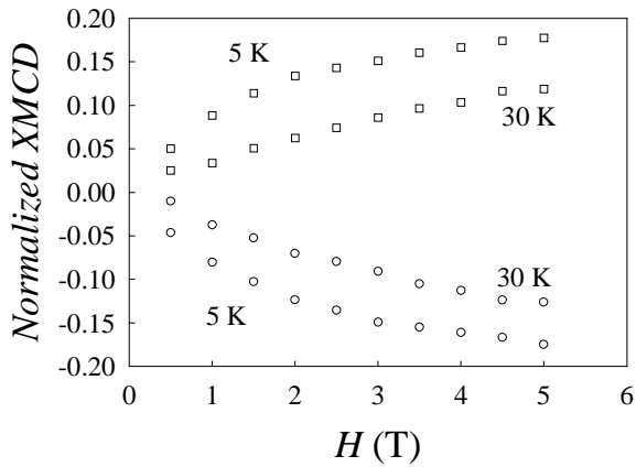
Fig. 1 – Normalized XMCD intensity for the peak at 642 eV (circles) and 643.5 eV (squares) in Mn12 as a function of H and at different temperatures.
