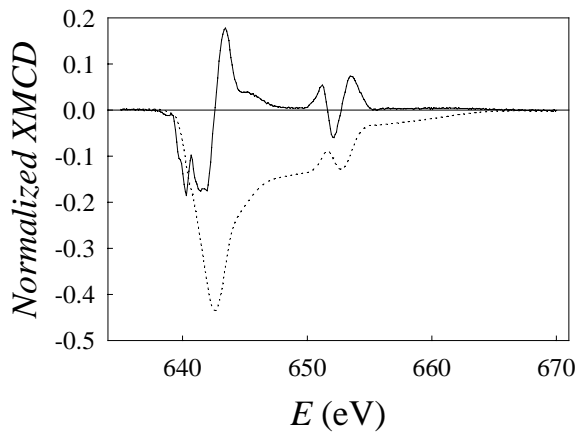
Fig. 3 – XMCD signal, normalized at unit white line intensity at the L-III edge for the Mn12 compound (full line). The field is 5 T and temperature is 5 K. The dotted line is the integrated XMCD. By direct comparison with the XAS spectra of Mn_2O_3 and MnO_2 , the peaks between 640 and 642.5 eV are attributed to Mn(III), while the peak at c.a. 643.5 eV is attributed to Mn(IV).
