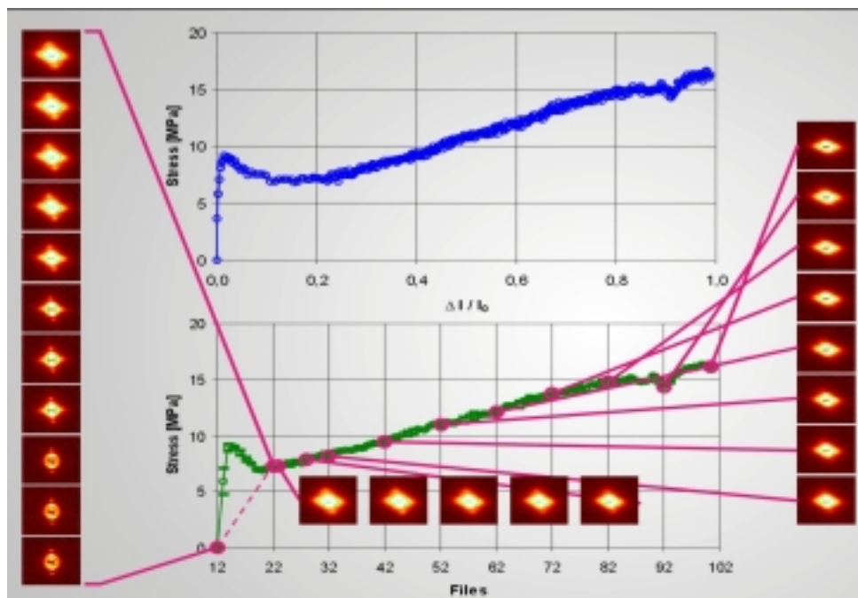
Fig. 2: Normal orientation of the lamellae to the stress field
