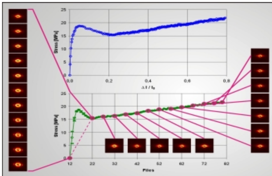
Fig. 1: Parallel orientation of the lamellae to the stress field
