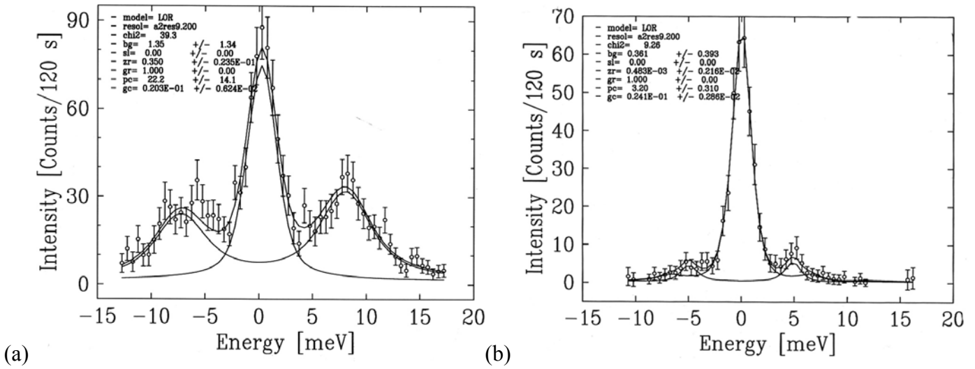
Figure 1: (a) spectrum obtained with sample A at 13.5 GPa at 17.8 keV ( \text{Si}_{999} ), at Q=(1.1, 1.1, 0) , \Delta E=7.7\pm 0.2 meV. (b) spectrum obtained with sample B at 16 GPa at 21.7 keV ( \text{Si}_{111111} ), Q=(1.06, 1.06, 0) ; \Delta E=4.61\pm 0.1 meV.
