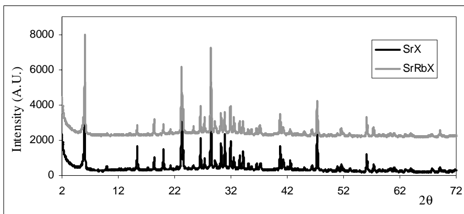
Fig. 1 : X-ray diagrams for hydrated SrX and SrRbX (recorded on a D501 Siemens diffractometer using K\alpha_1 and K\alpha_2 copper radiations)
