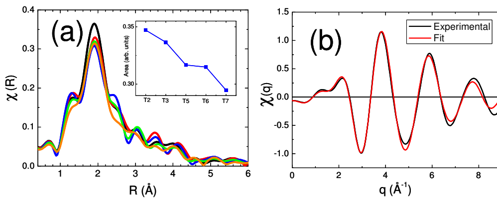
Figure 7. (a) Radial distribution function \chi(R) (colour code identical to figure 7). Inset shows the area of the first coordination shell as a function of the sensor (b) Fit of the \chi function in the q space with a tetrahedral coordination shell of oxygen atoms at 2.10 \text{\AA} .
