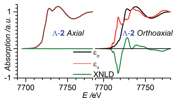
Fig. 4 XANES and XNLD obtained with linearly polarized X-rays for (a) axial ( \theta = 0^\circ ) and (b) orthoaxial ( \theta = 90^\circ ) configurations.
