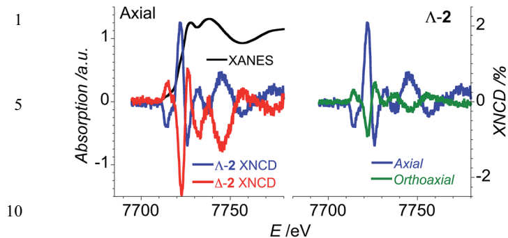
Fig. 5 (a) XANES (black) and XNCD spectra obtained in axial configuration ( \theta = 0^\circ ) for \Delta -2 (red) and \Lambda -2 (blue); (b) comparison axial (blue) and orthoaxial (green) XNCD spectra for a crystal of \Lambda -2.
