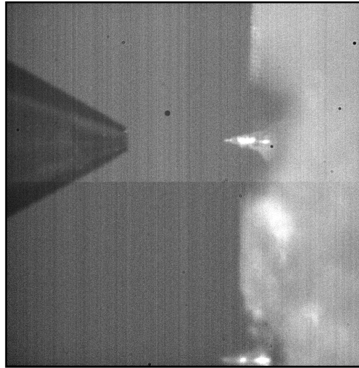
Figure 2 – Optical microscope image of diamond flat punch (left) approaching a micropillar (right)
