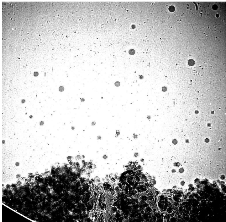
Figure 3. In situ build process showing a crack forming at the bottom
