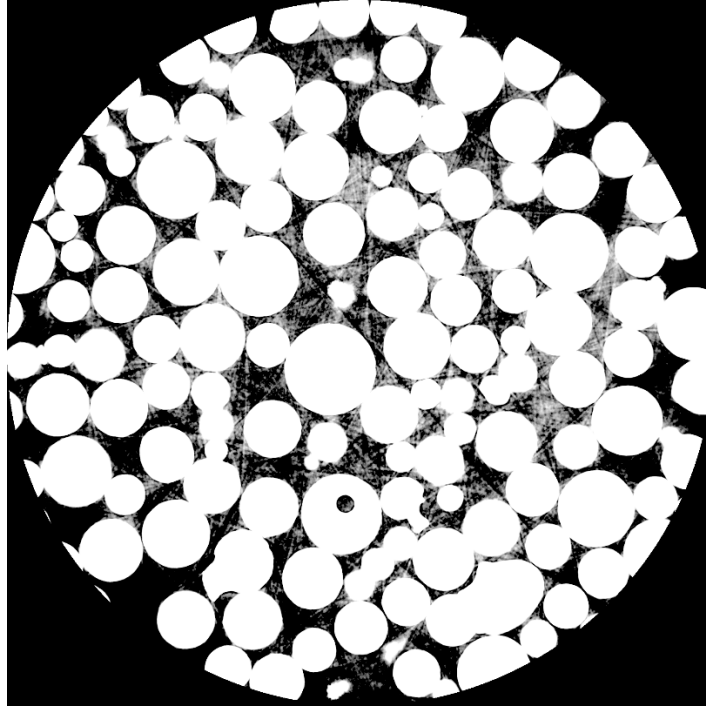
Figure 2. Reconstructed slice of the powder tomography scan showing powder geometry distribution
