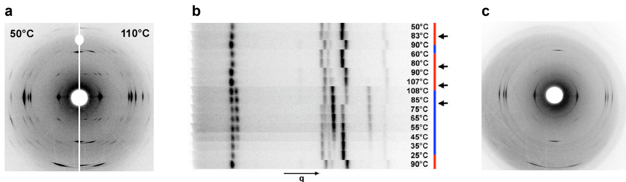
Figure 6. a) Two examples of diffraction diagrams recorded on hydrated strips of a tube from a Lamellibrachia vent worm, at 300 bars, and corresponding to two forms of \beta -chitin at 50°C ( left-half ) and 110°C ( right-half ). b) Display of the equatorial reflections of \beta -chitin diffraction diagrams recorded during various thermal treatments of the same sample, at 300 bars. The red and blue vertical bands correspond to heating and cooling steps, respectively. The black arrows indicate phase transitions. c) Diffraction pattern of never-dried Raftia \beta -chitin in environmental conditions (20°C, 300 bars).
