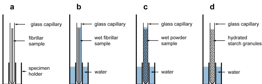
Figure 2. Sample set-up in the case of fibrillar (a,b) and powder specimens (c,d). The height of the specimen holder is about 2 cm.
