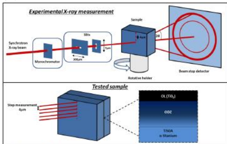
Figure 1: Synchrotron X-ray diffraction measurement and experimental method.
