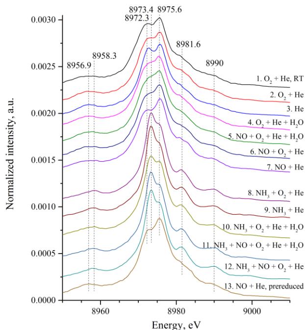
Fig. 3. XES spectra of Cu-SSZ-13 catalyst during NH 3 -SCR and under related model gas mixtures at 200 °C (exact composition and temperature given in the ESI, Table S2).
