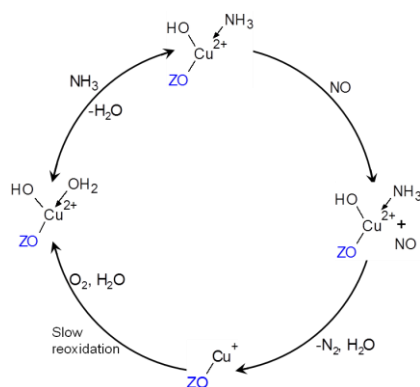
Scheme 1. Role of copper in Cu-SSZ-13 suggested by operando XES and XAS during NH 3 -SCR. Possible additional water / ammonia ligands are left out for clarity. ZO stands for zeolite cation-exchange site.
