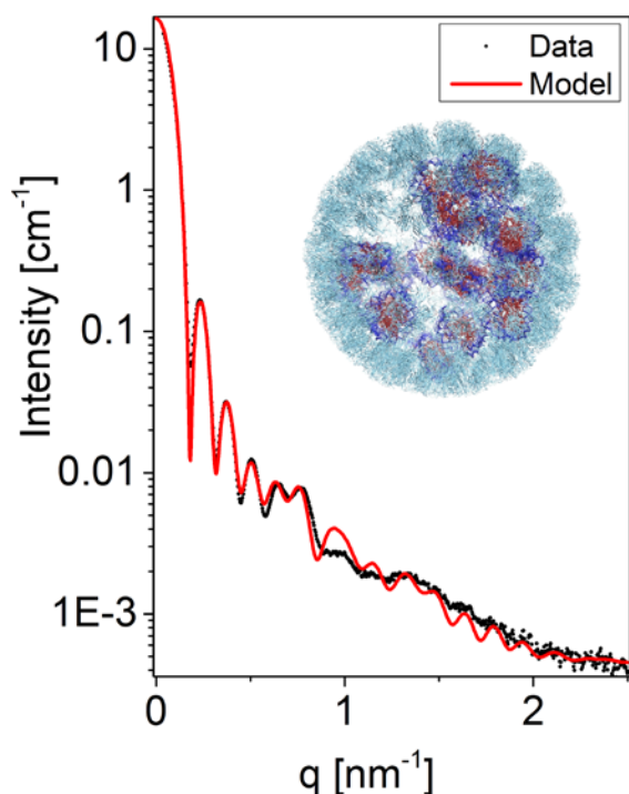
Figure 1. Scattering curve from wtSV40 and atomic model of the capsid and minichromosome (DNA and nucleosomes). Monte Carlo simulations were used to compute the most likely organization of the minichromosome and were verified against the ESRF SAXS data .
