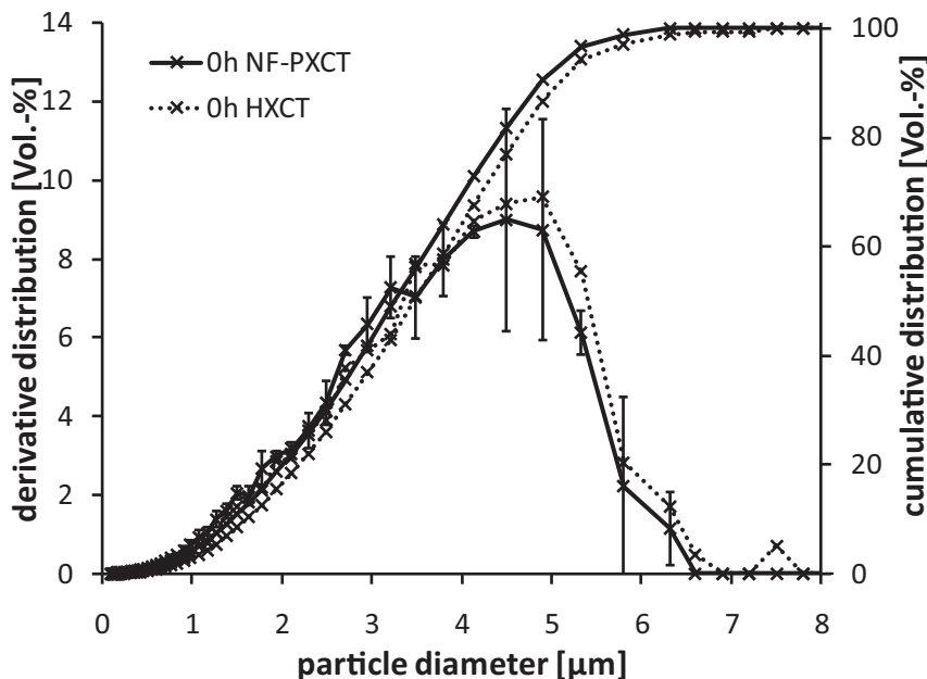
Fig. 6. Volume-based particle size distribution (cumulative and derivative) for HXCT and NF-PXCT measurements of anhydrous C_3S .
