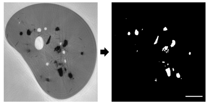
Fig. 4. Grayscale (left) and binary (right) images relative to a 2D section through the reconstructed volume (12-hours hydrated sample). Black: cement particles; grey: glue; white: air voids. Segmented C_3S particles in the binary image are shown in white. Scale bar: 10 \mu m.
