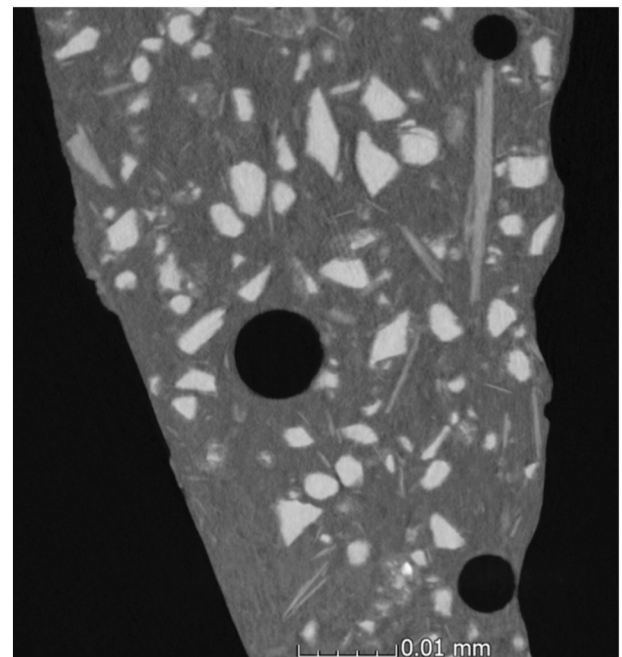
Fig. 5. 2D view of the C_3S sample hydrated for 12 h showing irregular shaped C_3S particles, elongated portlandite sections, C-S-H as a hydration rim around tricalcium silicate, epoxy resin and air (black).
