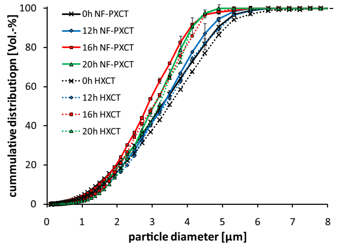
Fig. 7. Volume-based cumulative particle size distribution obtained from NF-PXCT and HXCT measurements of C_3S .
