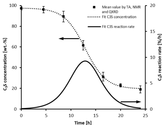
Fig. 2. C_3S concentration during 24 h of hydration given as the mean value from TA, NMR, and QXRD measurements (black squares) with its mathematical fit by Eq. (2) (dotted line), and C_3S reaction rate as the first derivative (multiplied by -1 ) of the C_3S concentration fit (bold line, right hand axis).
