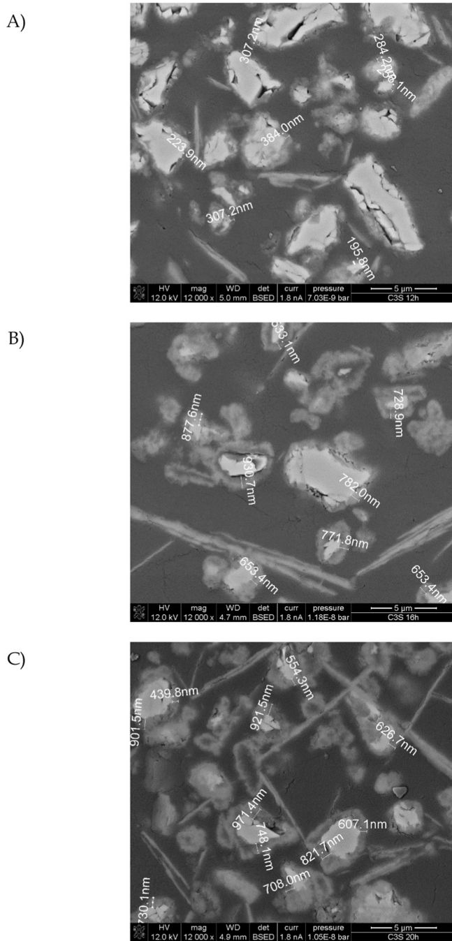
Fig. 3. SEM images of embedded samples hydrated for 12 h (A), 16 h (B), and 20 h (C) with measurements of the C-S-H layer thickness.
