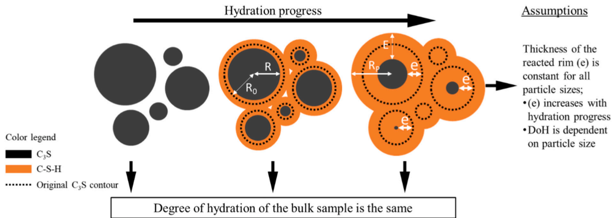
Fig. 1. ‘Reaction zone hypothesis’ for the development of the particle sizes of C_3S during hydration with individual degree of hydration of each particle size due to constant reacted rim thickness. R_0 -radius of the anhydrous particle, R -radius of the hydrated particle, e -reacted rim, E -C-S-H layer thickness, R_p -radius of the full particle (C 3 S core + C-S-H layer). The presentation focuses on details important to the present study; additional information such as formation of a gap between remaining C_3S cores and C-S-H or the difference between inner and outer C-S-H are not included to increase clarity of the presentation.
