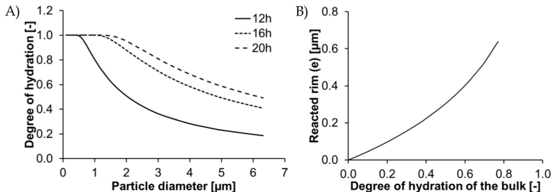
Fig. 8. Simulated degree of hydration of the C_3S particles in dependence of their size after 12 h, 16 h, and 20 h of hydration (A). Calculated reacted rim thickness of the C_3S particles in dependence on the degree of hydration (B).
