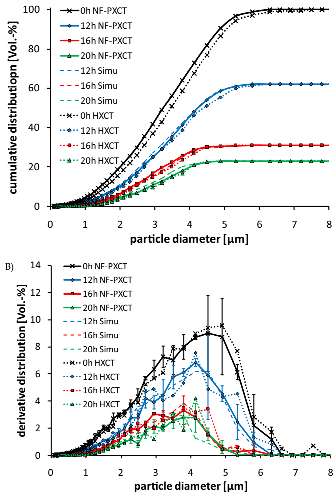
Fig. 9. Particle size distribution (A: cumulative, B: derivative) during C_3S -hydration. Measurement (NF-PXCT, HXCT) and simulation.
