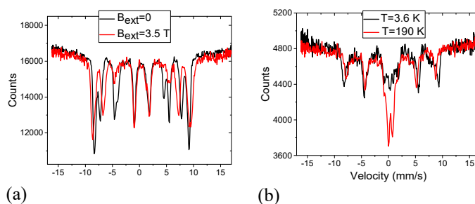
Fig.2. Mössbauer spectra for YFeO 3 thin films recorded at two applied fields at T = 3.5 K (a) and at two temperatures in zero magnetic field (b).
