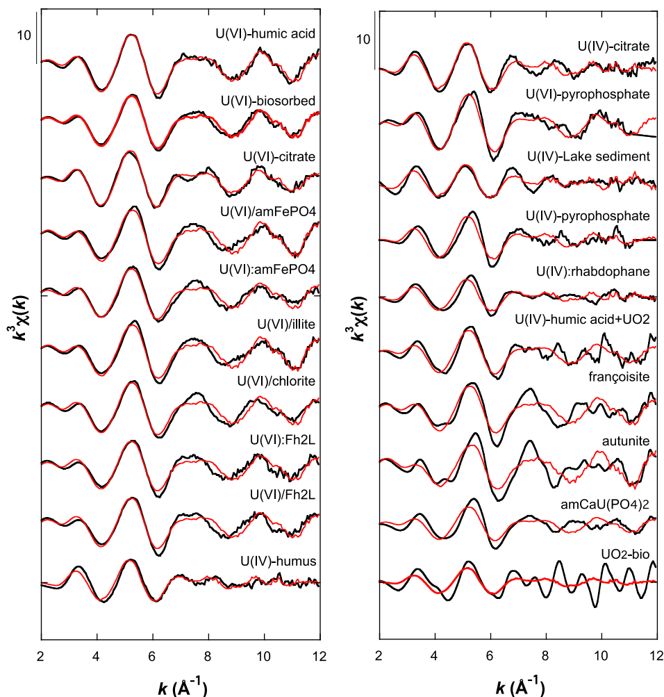
Fig. 9. Target Transform analysis of our set of model compounds U L_3 -edge EXAFS spectra, using the two first components of the PCA analysis of our wetland soil samples data. See Table S5 for quantitative results and for information and references on the reported model compounds spectra.
