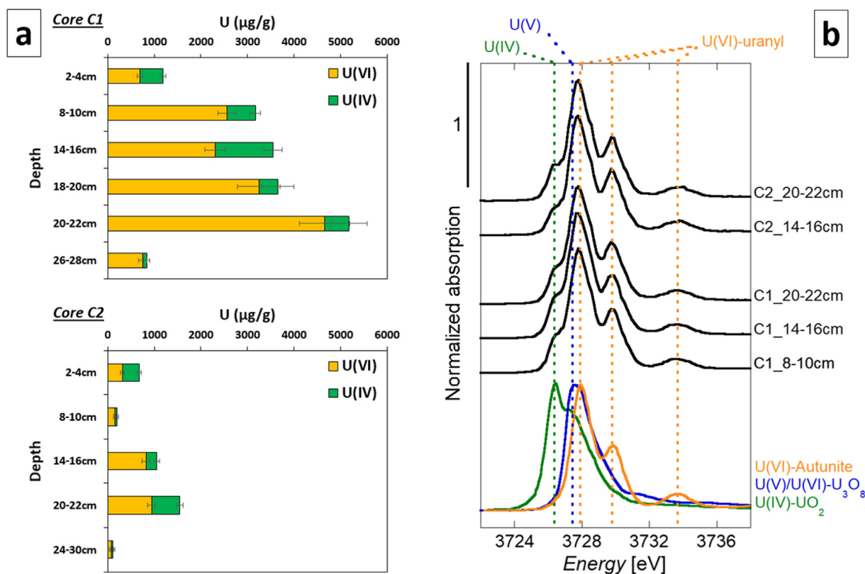
Fig. 8. Oxidation state of uranium in soil cores C1 and C2 determined by U L_3 -edge XANES and U M_4 -edge HERFD-XANES spectroscopies. (a) Depth profiles along cores C1 and C2 of the U(VI) and U(IV) contents (in \mu\text{g/g} ) determined from LC-LS fitting of U L_3 -edge XANES spectra. U(VI) concentrations are shown in orange, U(IV) in green. Error bars represent 3\sigma uncertainties. Fitting results are reported in Table 1. (b) HERFD-XANES spectra at the U M_4 -edge of reference compounds and soil samples from cores C1 and C2. Autunite was used as U(VI) reference, U_3O_8 contains 67 % U(V) and 33 % U(VI), and UO_2 was used as U(IV) reference (with a fraction of U(V)). Vertical dashed lines indicate the absorption features of U(IV) (green), U(V) (blue) and U(VI) (orange). (For interpretation of the references to color in this figure legend, the reader is referred to the web version of this article.)
