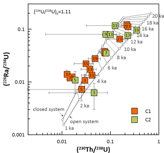
Fig. 13. Age constraints on U accumulation in soils of cores C1 (orange) and C2 (green) using radioactive disequilibria ( ^{230}\text{Th}/^{238}\text{U} and ^{226}\text{Ra}/^{238}\text{U} ). Authigenic activity ratios (corrected from detrital components) are plotted with Concordia curves corresponding to a closed system (upper curve) and an open system accounting for U and Ra losses (lower curve), with corresponding ages (in ky). The numbers in squares correspond to sample depths in the cores (in cm). See text for details on the open system model. (For interpretation of the references to color in this figure legend, the reader is referred to the web version of this article.)
