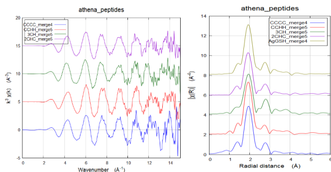
Figure 1. Experimental EXAFS spectra of Ag-substituted Zn-finger proteins in the reciprocal (left) and in the real space (right). For comparison, the spectrum of a AgGSH reference compound is reported (right panel, khaki yellow curve).
