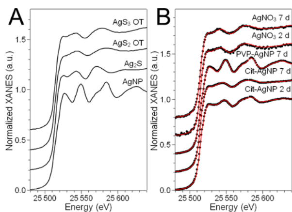
Figure 2. (A) XANES spectra of AgNP and of three Ag-S reference compounds: Ag-organothiol (OT) in trigonal and digonal coordination (AgS 3 and AgS 2 , respectively), and mineral acanthite (Ag 2 S). (B) Experimental XANES spectra (black dots) of selected samples measured in this experiment: 3D cultures of hepatic cells exposed to Ag nanoparticles or salt for 2 or 7 days, and best fitting curves (red) obtained as linear combination of the reference compounds reported in panel A.
